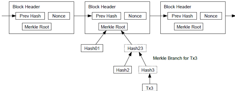
Longest Proof-of-Work Chain
